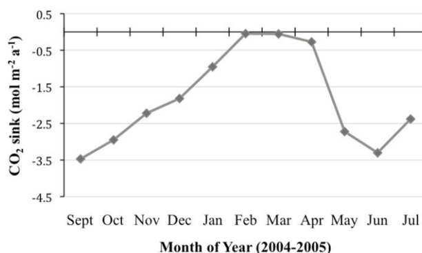
Figure 5 Monthly air-sea CO 2 fluxes at Northwest K1 CELAS time series site
