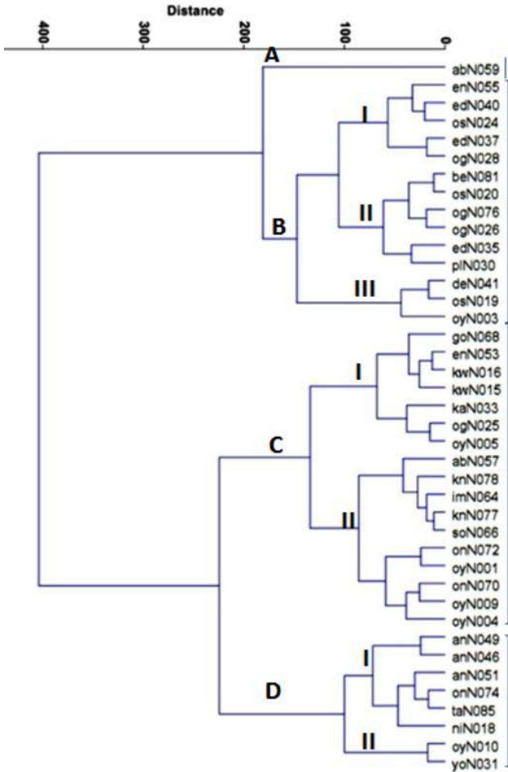
Fig. 3. Cluster analysis based on morphological characters.
