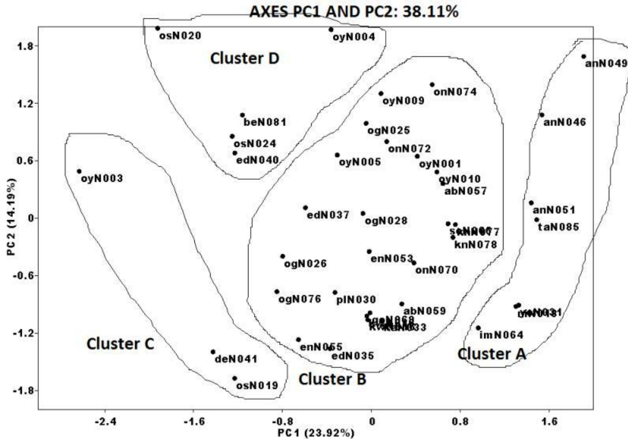
Fig. 2. A two dimensional plot of Principal Components Analysis of the 40 accessions of Moringa oleifera based on normalized variance-covariance matrix using PAST software 2013.
