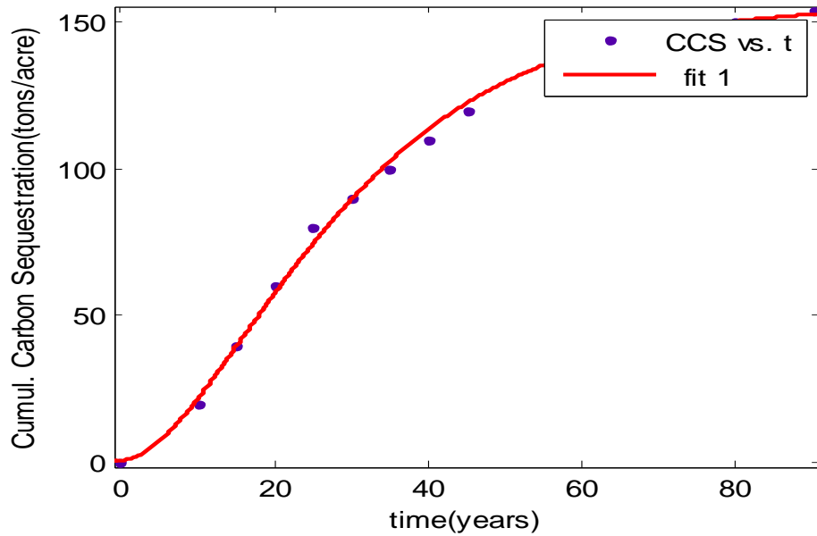
Fig.1a; Cumulative Carbon Sequestration versus time, model 1
