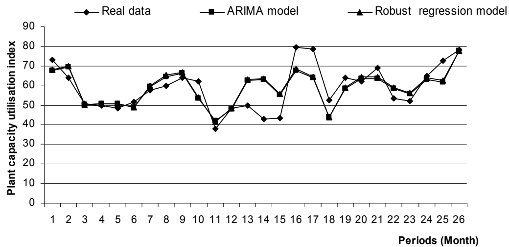
Figure 6 Comparison of prediction values for the plant capacity utilisation index using the in-sample datasets.
