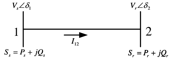
Figure 2: Typical one-line diagram of transmission line.
