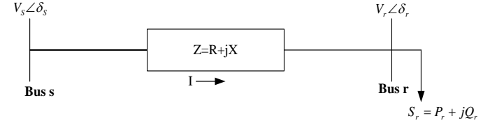
Figure 3: One-line diagram of a two-bus power system model
