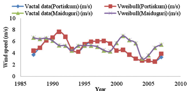
Fig. 8. Plot showing the predictive ability of the Weibull distribution for yearly mean wind speed distribution.
