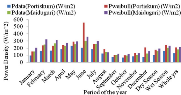
Fig. 9. Plot showing the power density distribution for both measured data and Weibull result for the two stations for particular period of the 21 years considered.
