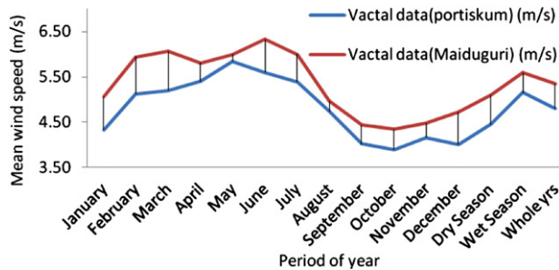
Fig. 12. Plot comparing measured mean wind speed for the two sites based on specific period of the 21 years.
