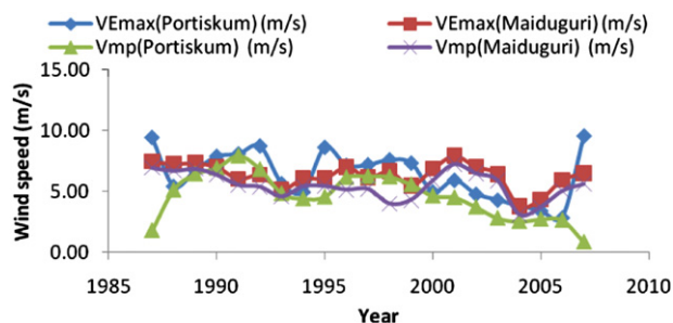
Fig. 14. Plot comparing the yearly most probable and maximum likelihood wind speeds for the two sites based for the 21 years period.
