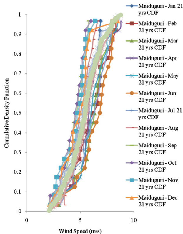
Fig. 5. CDF Plots for Maiduguri.
