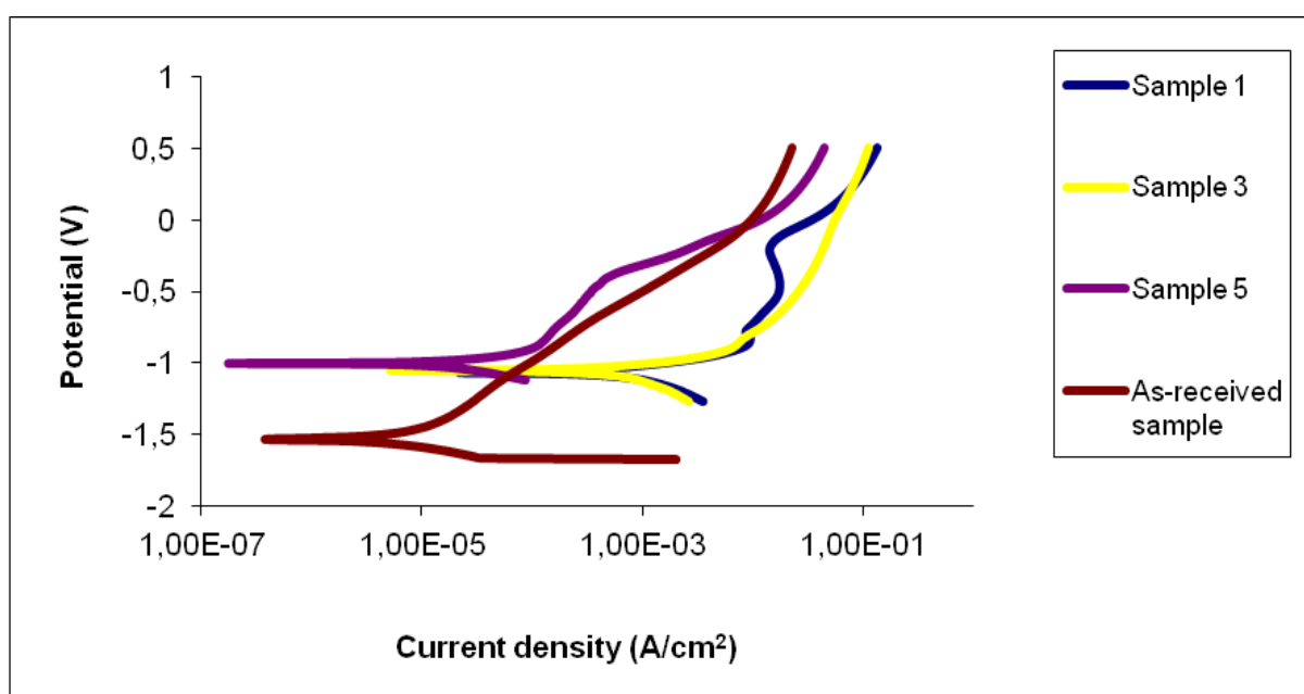
Figure 19. Potentiodynamic polarization curves for Zn deposited mild steel
