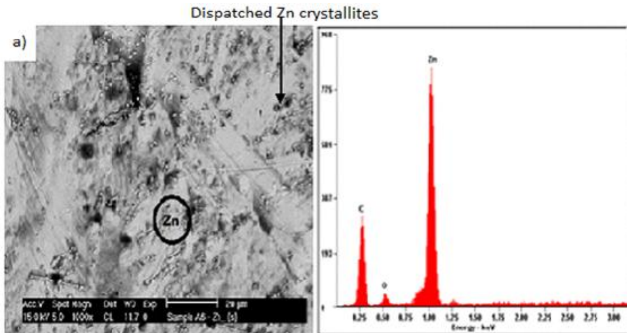
Figure 12. SEM/EDS of Zn 3 showing the surface morphology of the deposited sample
