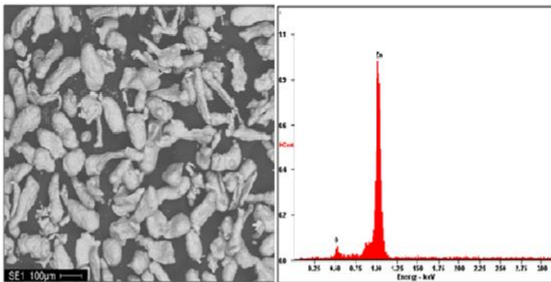
Figure 3. SEM/EDS spectra Zn
