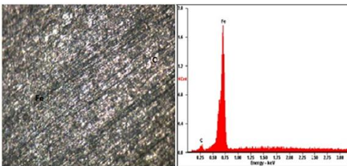
Figure 1. Optical Micrograph and EDS of as-received mild steel
