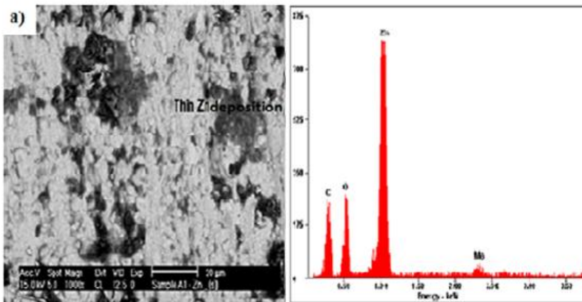
Figure 10. SEM/EDS of Zn 1 showing the surface morphology of the deposited sample
