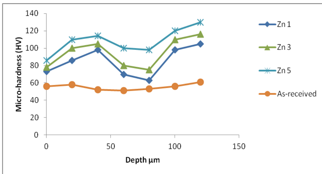
Figure 13. The microhardness/depth profile for zinc deposited sample
