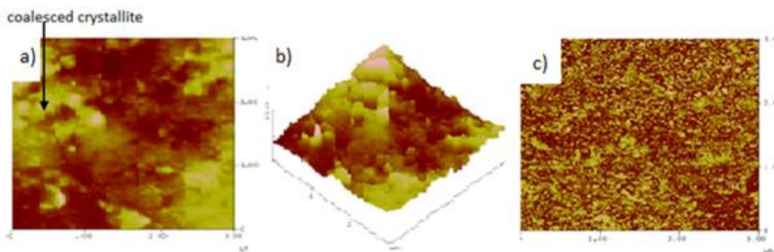
Figure 5. AFM images of the Zn film obtained for sample 2; (a) 2-D image, (b) 3-D relief image and (c) roughness analysis
