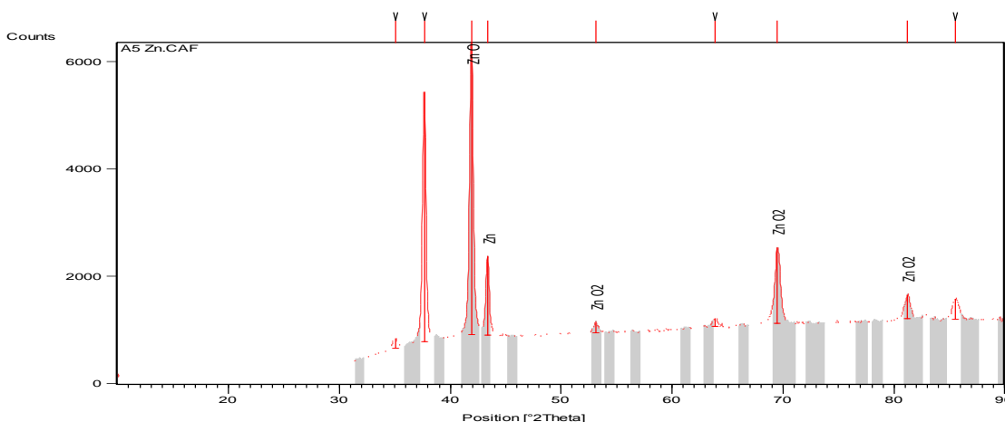
Figure 9. Solid X-ray diffraction profile for Zn 3
