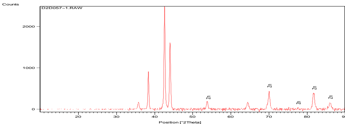
Figure 7. Solid X-ray diffraction profile for Zn 1
