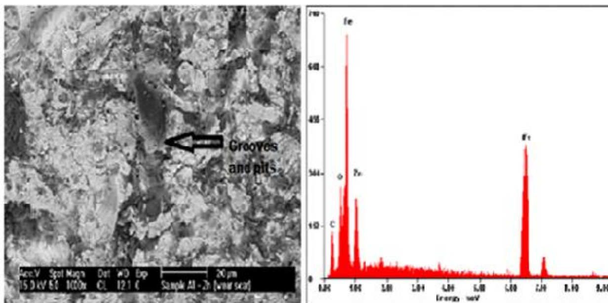
Figure 16. SEM/EDS spectra of the wear scar on Zn 1
