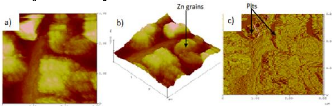
Figure 21. AFM images of the surface film obtained for Zn 1 after corrosion
