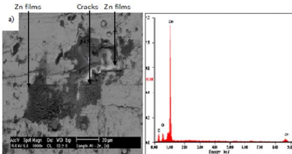
Figure 11. SEM/EDS of Zn 2 showing the surface morphology of the deposited sample.
