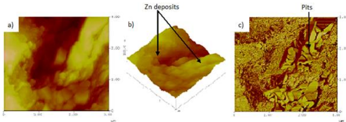
Figure 21. AFM images of the surface film obtained for Zn 1 after corrosion
