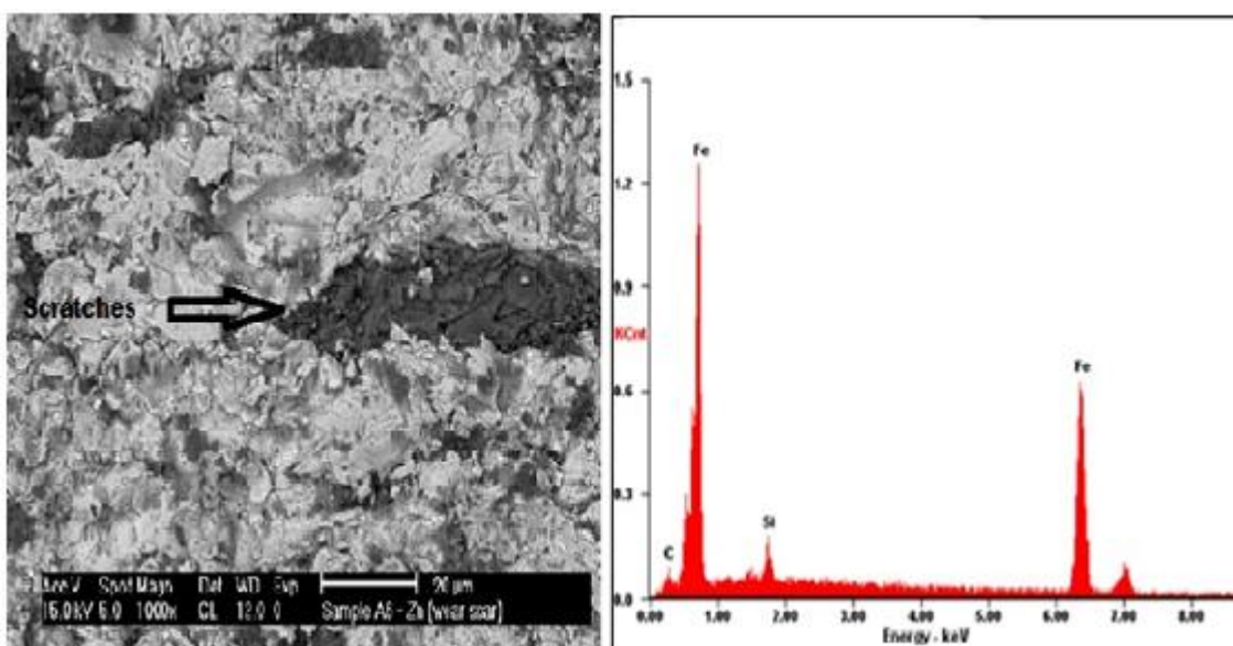
Figure 18. SEM/EDS spectra of the wear scar on Zn 3
