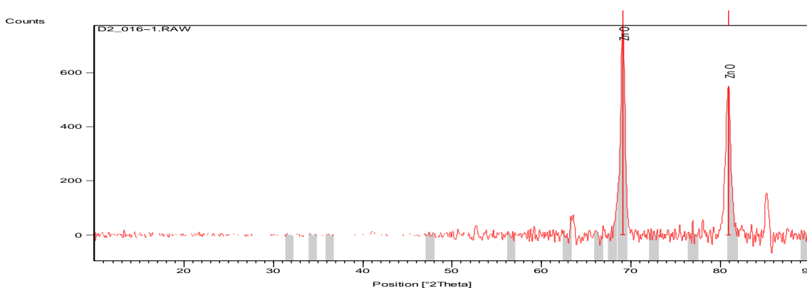
Figure 8. Solid X-ray diffraction profile for Zn 2
