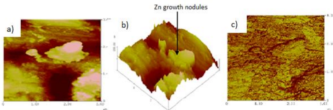
Figure 4. AFM images of the Zn film obtained for sample 1; (a) 2-D image, (b) 3-D relief image and (c) roughness analysis
