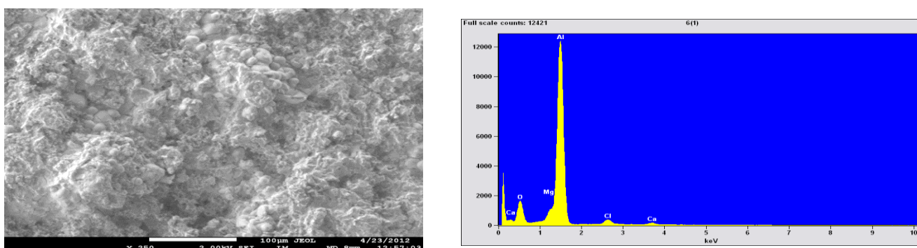
Figure 9. SEM micrograph of aluminium in 50% v/v Ricinus communis -2M HCl solution after 36 h exposure time with the EDS
