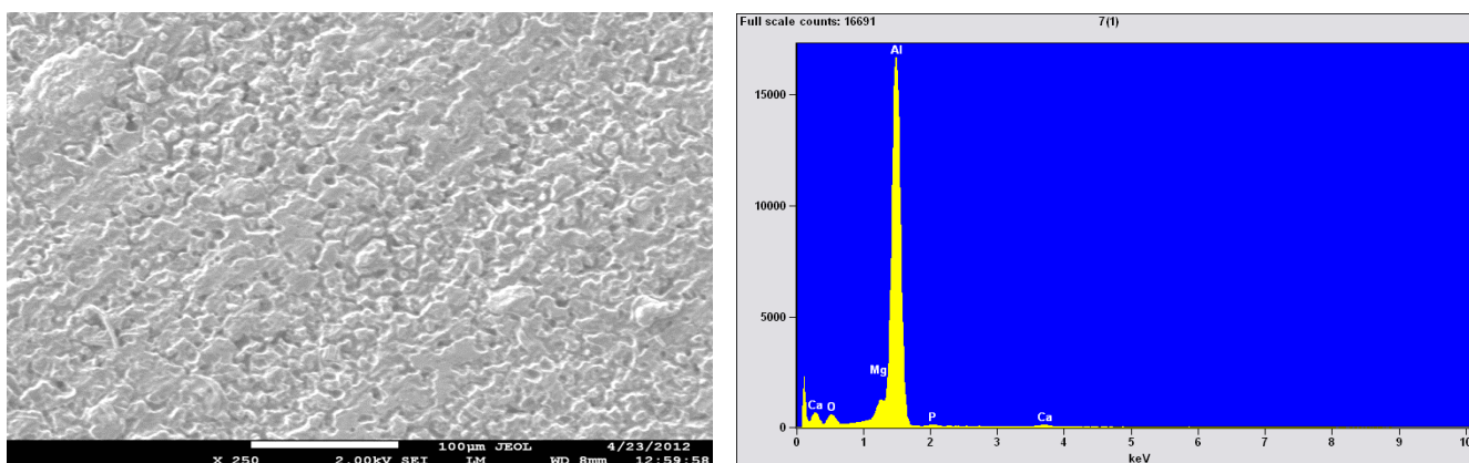
Figure 10. SEM micrograph of aluminium in 50% v/v Ricinus communis -2M H 3 PO 4 solution after 36 h exposure time with the EDS
