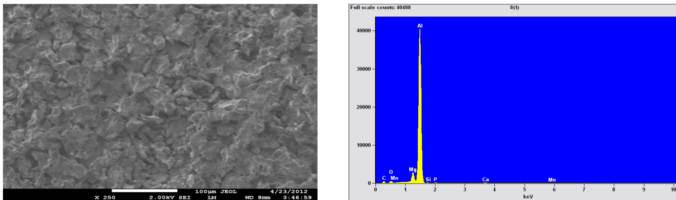
Figure 8. SEM micrograph of aluminium in uninhibited 2M H 3 PO 4 solution after 12 h exposure time with the EDS
