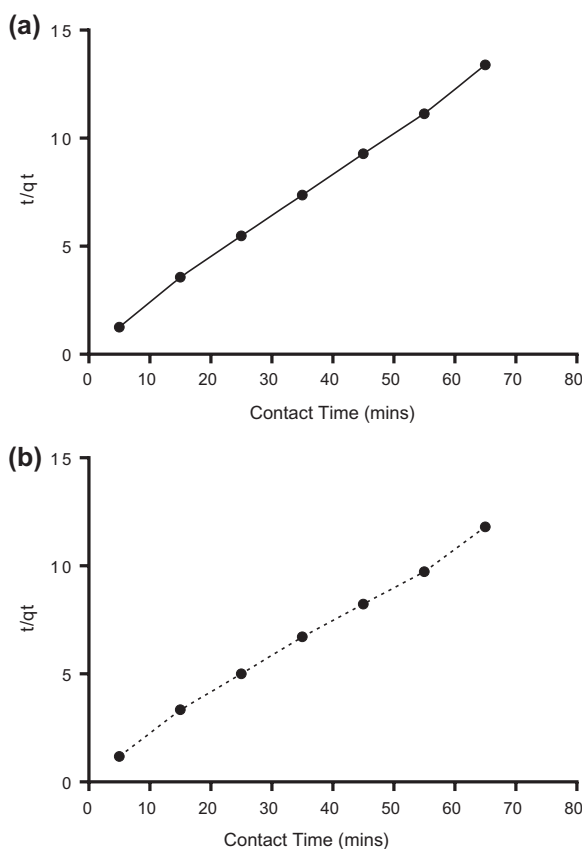
Figure 6. Plot of pseudo second-order kinetic model for Cu adsorption using KOH-activated UmpP; 150 mg/L initial Copper concentration, 0.4 g biomass, pH 5.5 at 800 rpm (a) 303 K (b) 308 K.
