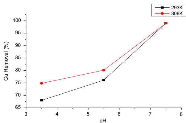
Figure 1. Copper removal by KOH-activated UmpP (0.4 g in 20 mL) influenced by pH of the solution (100 mg/L Cu concentration) at varied temperature.
