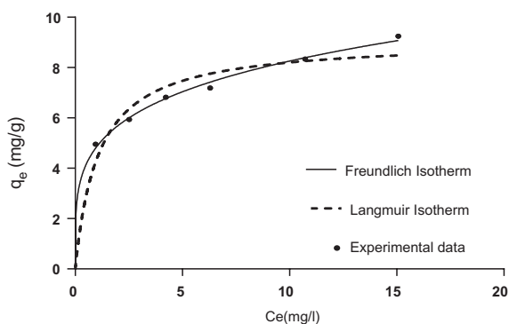
Figure 4. Equilibrium isotherm at 303 K.
