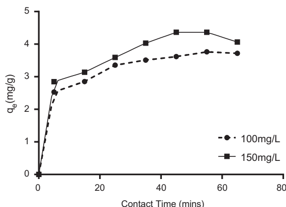
Figure 3. Copper removal by KOH-activated UmpP (0.4 g in 20 mL) as affected by initial concentration (100 and 150 mg/L Cu concentration) and contact time.
