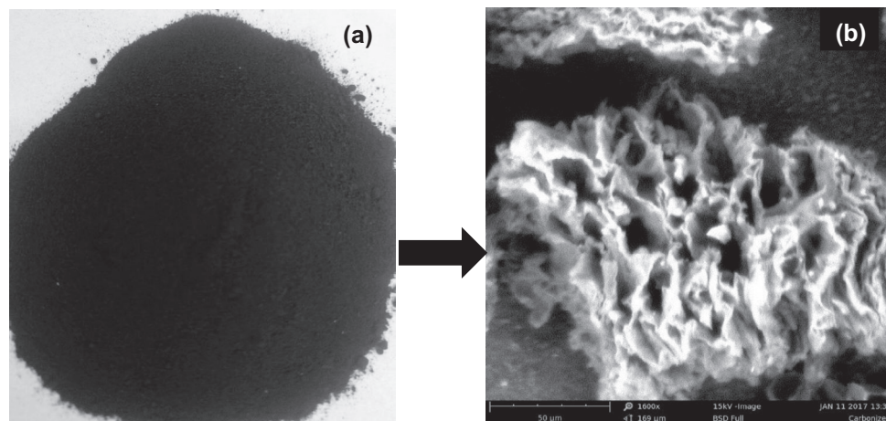
Plate 1. KOH-activated Musa paradisiaca peel (a) Granular sample (b) SEM image.
